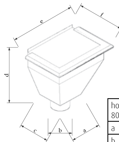
Hopper head
